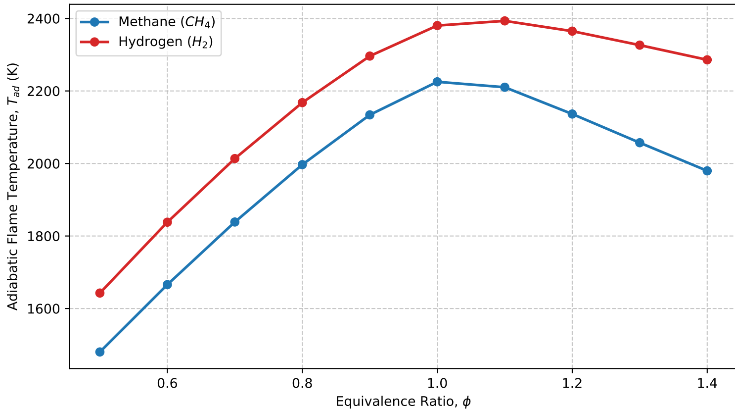
a) Adiabatic Flame Temp vs Equivalence Ratio (Baseline: T_{in}=300\text{K} , P=1\text{ bar} )
